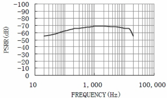
PSRR vs Frequency VDD=5V, RL=8Ω, Input 10Ω terminated
