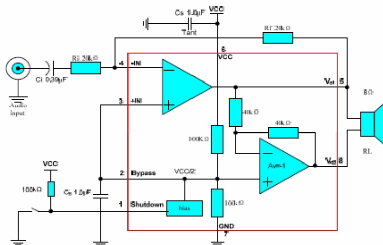
Typical Audio Amplifier Application Circuit
