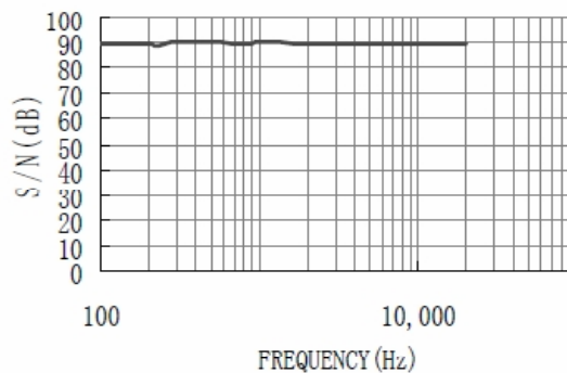
S/N vs Frequency T=25°C, Vdd=3.3V, RL=4Ω, and Po=425mW
