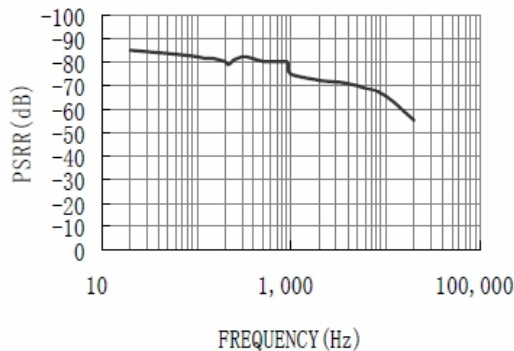
PSRR vs Frequency VDD=5V, RL=8Ω, Input Floating
