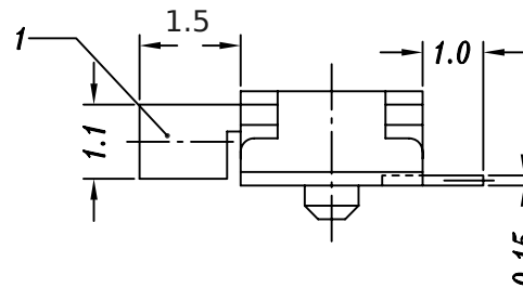
Slide Switch SMD Horizontal - 4 pins - 1 circuits - 3 positions
