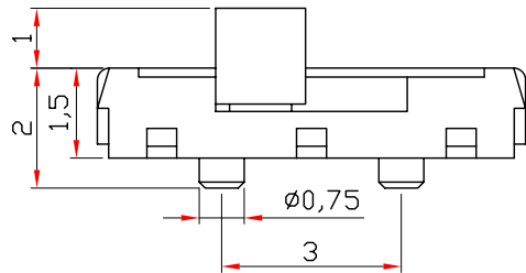
Slide Switch SMD Vertical - 6 pins - 2 circuits - 2 positions https://www.sunrom.com/m/7499
