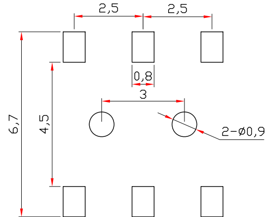
PCB Foot Print - Top View
