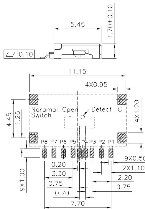
Recommended P.C.B. Layout (PCB Board Tolerance±0.05)
